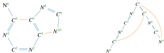
Fig. 2: Hydrogen-suppressed molecular graph of adenine ( C_5H_5N_5 ) and corresponding spanning tree with cycle edges (dotted); subscripts indicate correspondence of vertices
