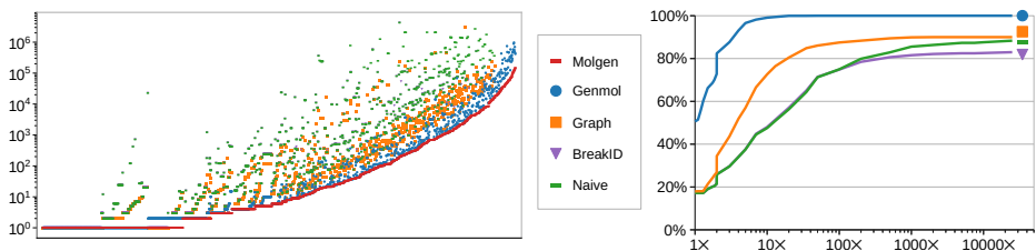
Fig. 3: Number of models for each compound in the data set (left) and ratio of compounds with model counts within a factor of the gold standard (right)
