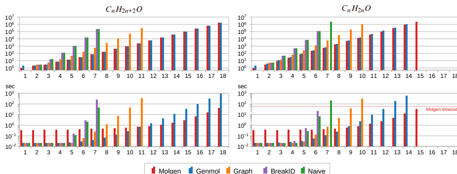
Fig. 4: Model numbers (top) and runtimes (bottom) for molecules of increasing size
