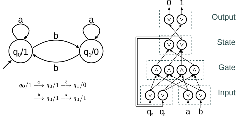
Figure 2. A simple Moore-machine, the processing of the input word abba (left) and a corresponding McCulloch-Pitts-network (right).
