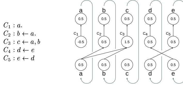
Figure 5. A simple propositional logic program and the corresponding network. Numbers within the units denote the thresholds. All weights are set to 1.
