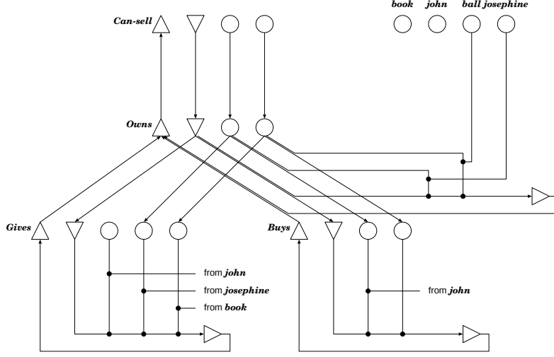
Figure 4. A SHRUTI network for the knowledge base from Table 2. Each predicate is represented by two relais units ( \Delta, \nabla ) and a set of argument units ( \bigcirc ). Constants are represented as \bigcirc -units in the upper right. Facts are implemented using \triangleright -units.
