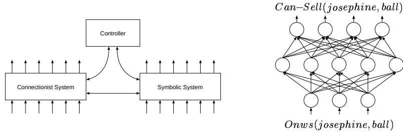
Figure 10. Hybrid (left) versus integrated (right) architecture.
