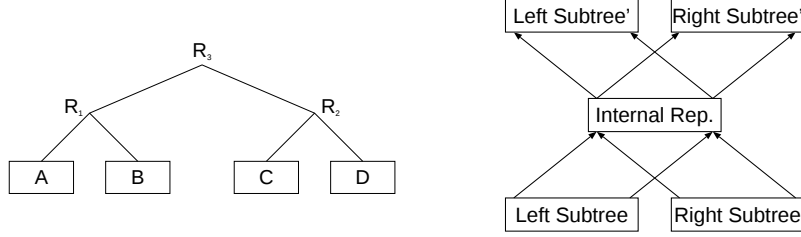
Figure 3. Example tree and a RAAM for binary trees.
